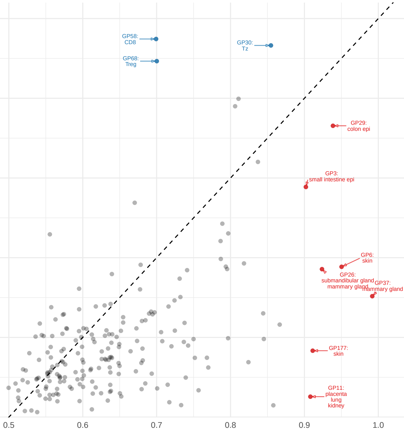
Max AUC: Organ vs Level-1
